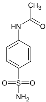
Sulfanilamid:
