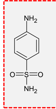
Sulfanilamid
