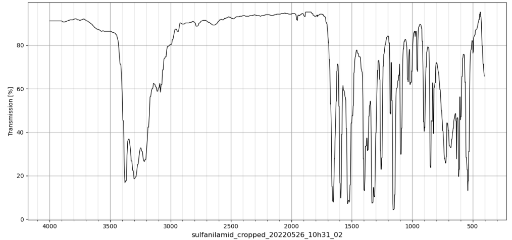
p-Acetamidobenzensulfonamid:
